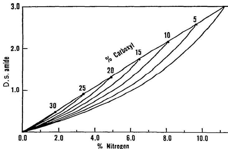
Fig. 1. D.s. by amide vs. percent of nitrogen at various percentages of carboxyl group for O -(carbamoylethyl)- O -(carboxyethyl)cellulose.
